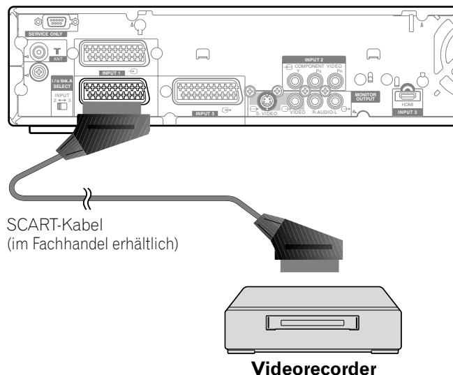
Videorecorder
